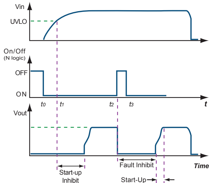
Figure E: Power Up/Down Diagram showing Start-Up Inhibit Period (not to scale)
