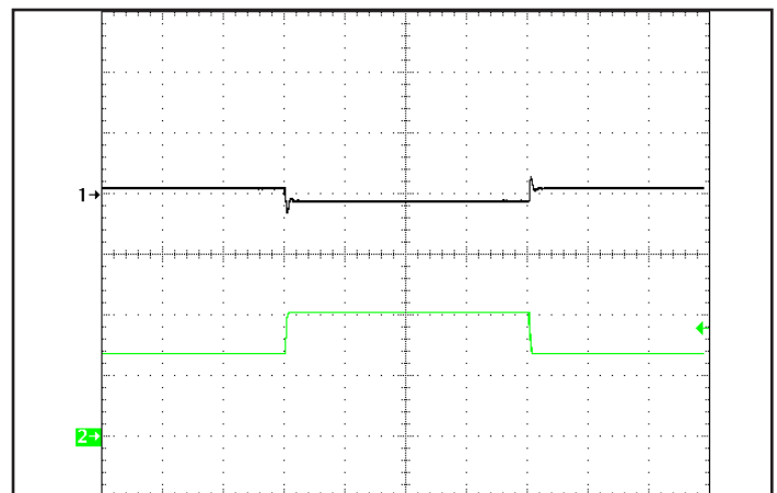
Figure 12: Output voltage response to step-change in load current (50%-75%-50% of I_{out(max)} ; dI/dt = 1A/\mu s ). Load cap: 15µF, 30 mΩ ESR tantalum cap and 1µF ceramic cap. Ch 1: V_{out} (1V/div), Ch 2: I_{out} (25A/div).
