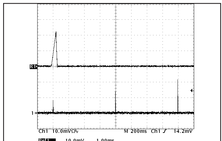
Figure 18: Load current (50A/div) as a function of time when the converter attempts to turn on into a 1m\Omega short circuit. Top trace (1ms/div) is an expansion of the on-time portion of the bottom trace.
