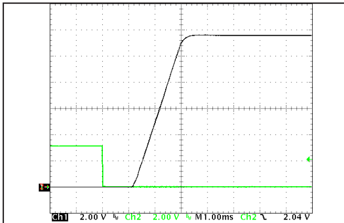
Figure 9: Turn-on transient at half load (resistive load) (1 ms/div). Load cap: 15µF tantalum capacitor and 5mF ceramic capacitor bank. Input voltage pre-applied. Ch 1: V_{out} (2V/div). Ch 2: ON/OFF input (2 V/div).
