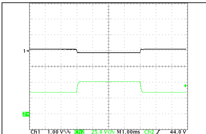
Figure 11: Output voltage response to step-change in load current (50%-75%-50% of I_{out(max)} ; dI/dt = 0.1A/\mu s ). Load cap: 15µF tantalum cap and 1µF ceramic cap. Ch 1: V_{out} (1V/div), Ch 2: I_{out} (25A/div).
